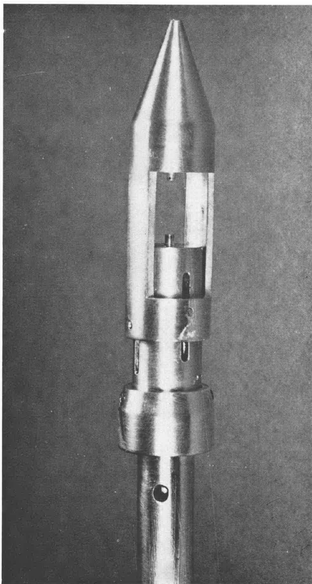
Figure 2. Photograph of a compression apparatus. This is not the apparatus actually used but differs only slightly in some absolute and relative dimensions.
